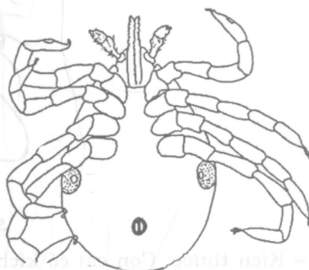
Ixodes haxagonus
