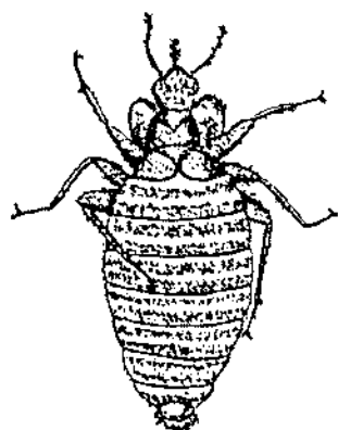
Cimex lectularius
