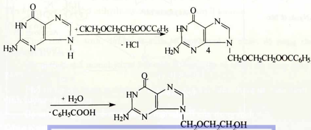
Acyclovir
