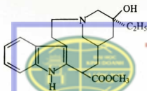
Catharanthin
