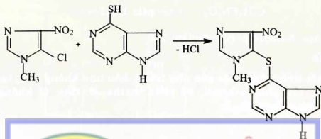
Azathioprin
