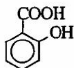
Acid o-hydroxy benzoic
