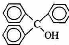
Triphenyl carbinol
