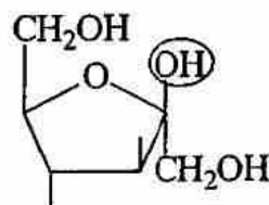
\beta -D-fructofuranose
