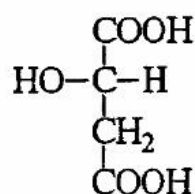
acid L(-) malic
