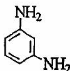
m-Phenylen diamin
