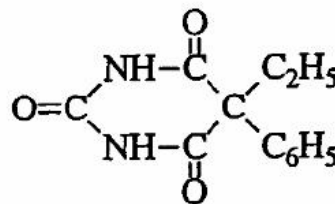
Acid 5-ethyl-5-phenyl barbituric (Luminal)
