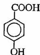
Acid p-hydroxy benzoic
