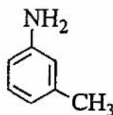
m-Toluidin
