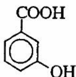
Acid m-hydroxy benzoic
