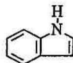
Benzopyrrol (indol)
