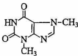
Theobromin
