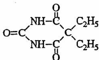
Acid 5,5-diethyl barbituric (Veronal)
