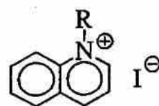
Alkylquinolini iodid
