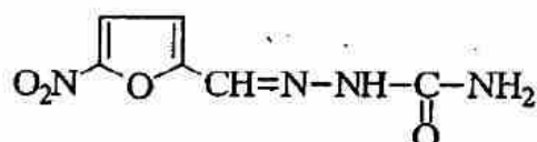
Nitrofurazon (5-nitro-2-furfuryliden semicarbazon)
