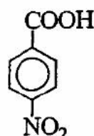
Acid p-nitro benzoic
