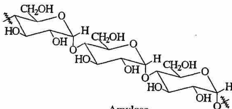
Amylose
