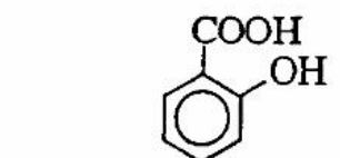
Acid o-hydroxy benzoic (acid salicylic)
