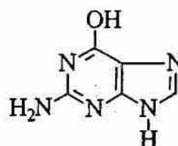
Guanin (2-amino 6-hydroxy purin)
