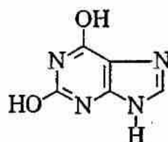
Xanthin (2,6-dihydroxy purin)
