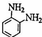
o-Phenylen diamin
