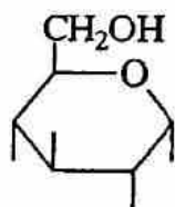
\alpha -D-glucopyranose
