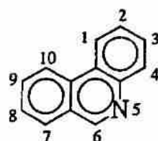
Phenantridin
