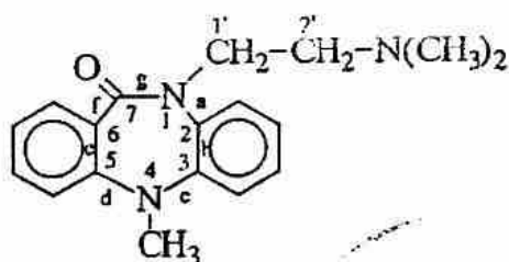
1-(2'-dimethylaminoethyl)-4-methyl-7-oxo dibenzo [b,e] 1,4-diazepin
