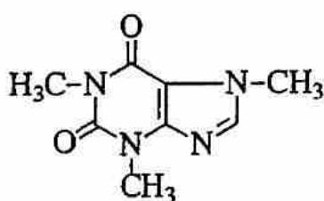
Cafein
