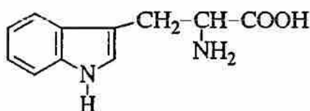
Tryptophan
