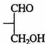
Aldehyd L-glyceric
