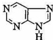
Purin
