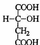
Acid D(+) malic
