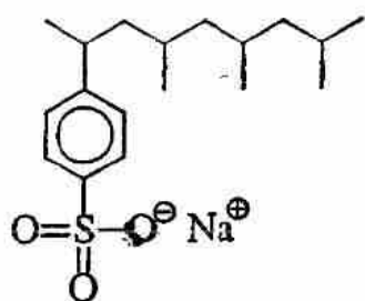
Natri alkyl benzensulfonat
