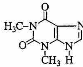
Theophylin
