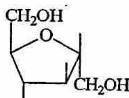
\beta -D-fructofuranose
