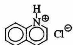
Quinolini clorid
