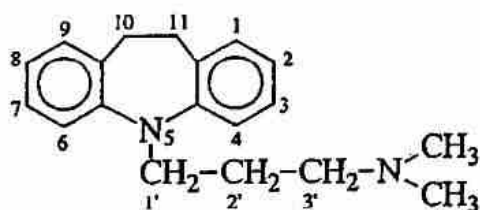
5-(3'-dimethylaminopropyl)-10,11-dihydro-5H-dibenzo [b,f] azepin (imipramin : chống trầm uất)
