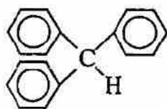
Triphenyl methan
