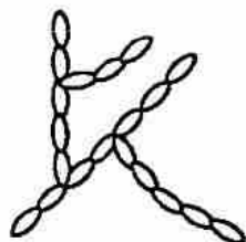
Amylopectin
