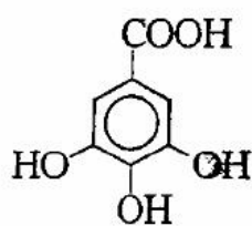
Acid galic
