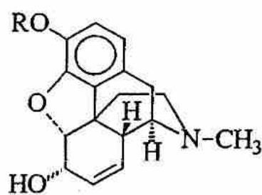
Morphin (R = H)
