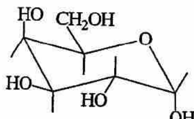
\alpha -D-galactopyranose
