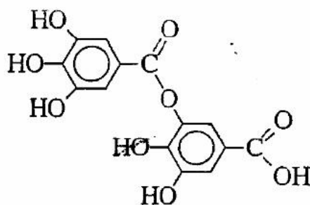
Acid metadigalic
