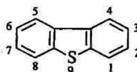
Dibenzothiophen
